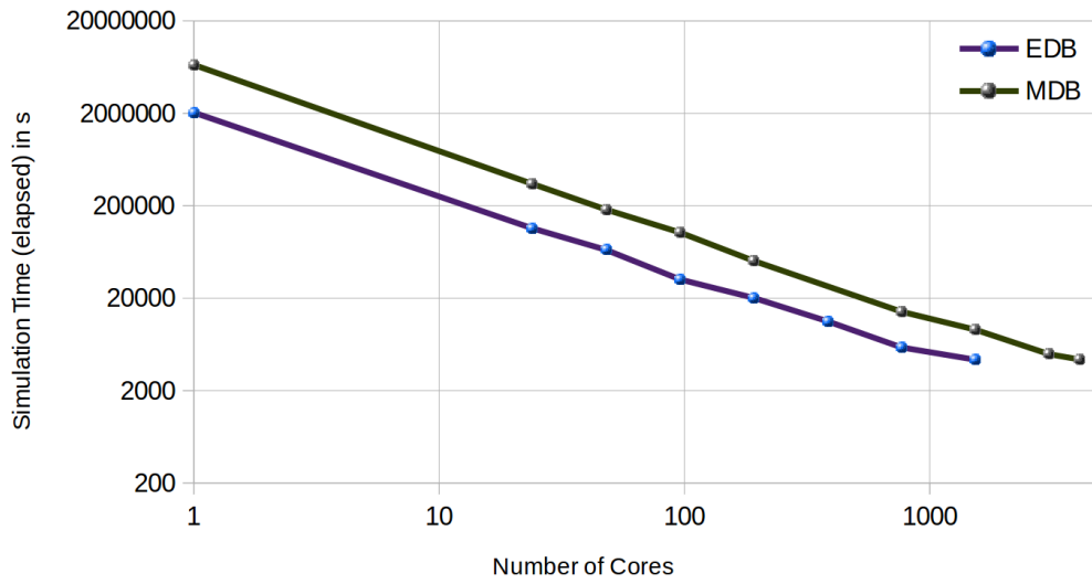
Fig. 5: Elapsed time for the explicit analysis (only the mechanical solver).
